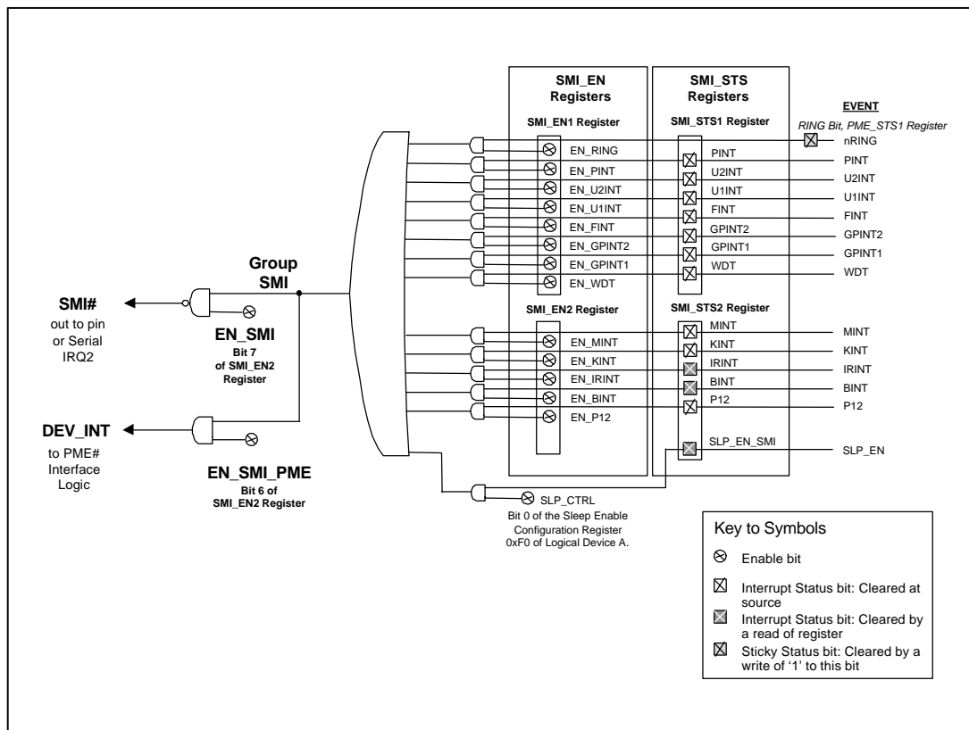
FIGURE 8 - SMI/PME LOGIC
