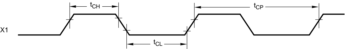
FIGURE 13-2. Clock Timing
