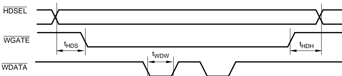
FIGURE 13-18. Write Data Timing
