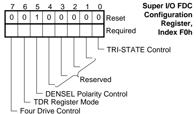
FIGURE 2-9. SuperI/O FDC Configuration Register Bitmap
