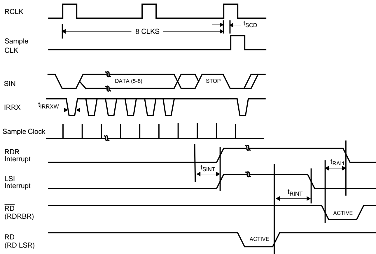
FIGURE 13-8. Receiver Timing
