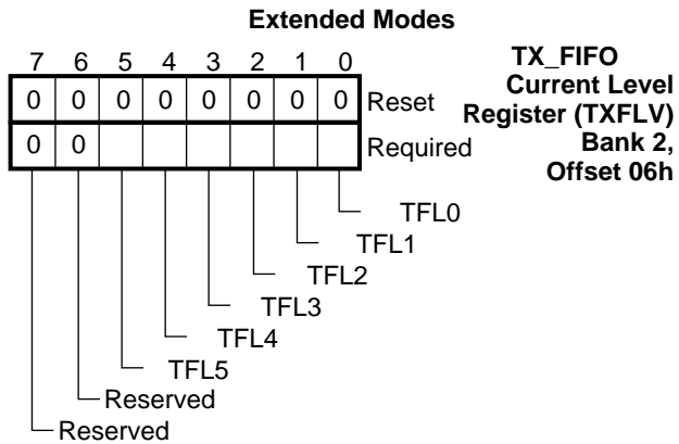
FIGURE 7-26. TXFLV Register Bitmap
